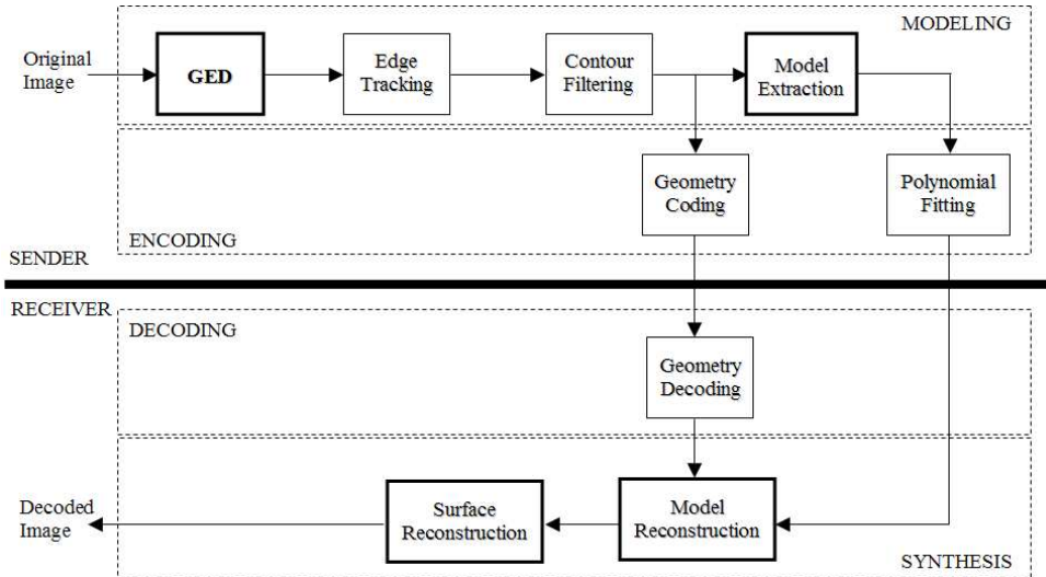
Figure 2. The generic architecture of the codec system.
